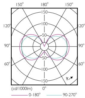
CorePro LEDcapsule MV 35W G9 830 Capsule
